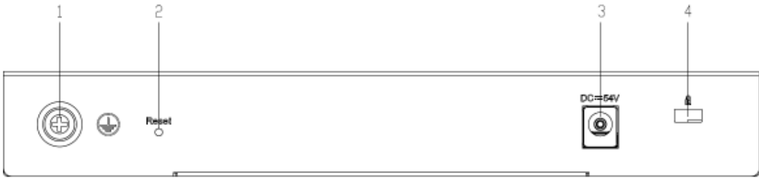
Figure 1-6 Back Panel of RG-ES209GC-P
