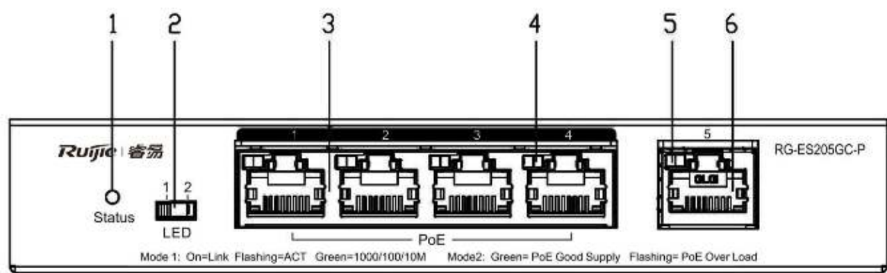
Figure 1-2 Front Panel of RG-ES205GC-P
